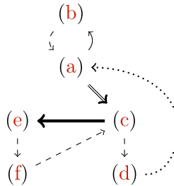
FIGURE 1. Logical connections between statements (a)–(f) in Remark 2.27. Dashed arrows: trivial implications which hold for any \mathcal{B} \subset \mathbb{N} \setminus \{1\} . Dotted arrow: this implication was explained in the paragraph before Theorem 2.18. Short plain arrow: implication follows from [4]. Thick arrow: this implication follows from Theorem 1.4. Double arrow: implication proved in Lemma 2.24.
