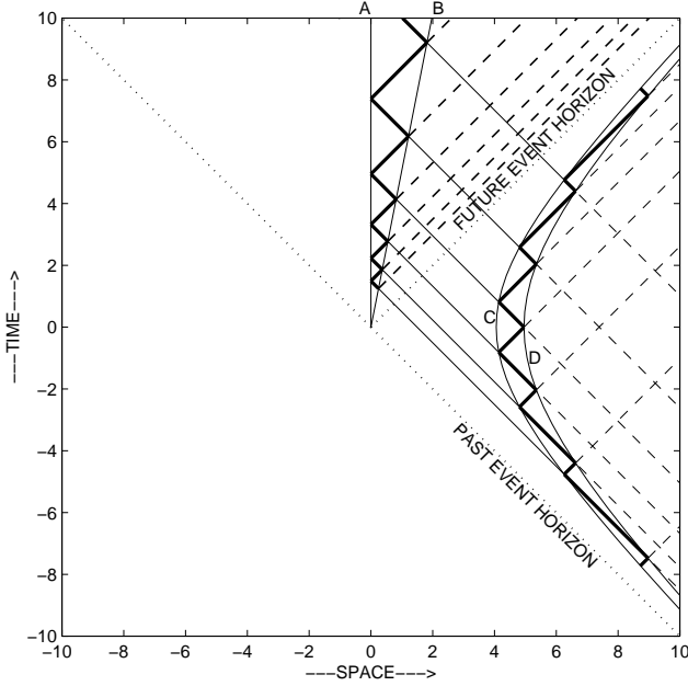
FIG. 12: One-way transfer of time from clock CD to clock AB. This transfer is achieved by the ticking of CD causing sympathetic tickings in clock AB. This process is brought about by e.m. pulses travelling from CD across the future event horizon to AB (solid thin 45° lines). They strike B at precisely the same rate and with the same phase as AB's clock pulse (heavy zigzag line) bouncing repeatedly off B.
