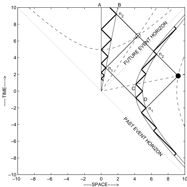
FIG. 13: Transfer of radar coordinates from clock CD to clock AB. The heavy dot in I gets mapped to the hollow dot in F . The radar coordinates of the event marked by the heavy black dot are the two clock pulses numbered n_1 and n_2 by accelerated clock CD. These two pulses cause CD to dispatch two pulses across its future event horizon. They are received by inertial clock AB where the numbering of its pulses is the same, namely, n_1 and n_2 . These are also the radar coordinates of the encircled event (“hollow dot”) in F . If this and other such events lie along the straight dashed line in F , then a free-float physicist who watches AB knows that the scattering source in I has the world line of the dashed hyperbola in I .
