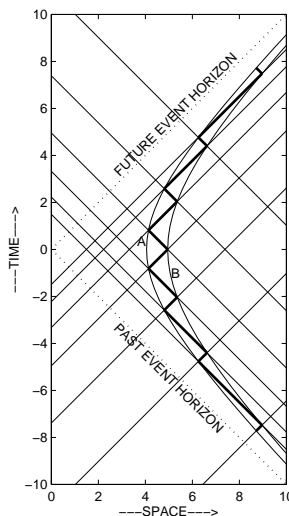
FIG. 3: Spacetime history of an accelerated clock and the null trajectories of trains of emitted and received pulses (light lines) whose emission and reception is controlled by the internal pulse (heavy line) bouncing back and forth between A and B.
