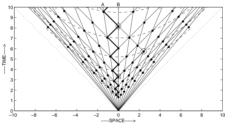
FIG. 9: Lattice of spacetime graduation events (heavy dots) determined and calibrated by a single geometrical clock AB which is expanding inertially. The spacetime history of the e.m. pulse bouncing inside this clock is the heavy zig zag line left of the middle. The clock is bounded by two straight lines A and B, the histories of the receding reflectors which keep the e.m. pulse trapped inside the clock. The other straight lines indicate the receding reflector histories of identically constructed clocks, if they were to form an array of adjacent geometrical clocks. The hyperbolas (dashed lines) are the times simultaneous with the tickings of the standard clock AB. The 45^\circ lines emanating to the left from A and to the right from B are the histories of the two trains of pulses escaping from A and B. The fact that AB is a standard clock implies that all graduation events of the calibrated lattice lie on these histories. Based on the method of pulsed radar, each graduation event (e.g. the encircled dot) is labelled by two unique integers, namely two numbered ticks (the dots in the square and in the diamond) of the clock. They are AB's "radar coordinates" of that graduation event.
