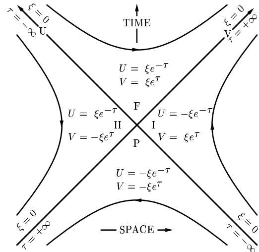
FIG. 1: Acceleration-induced partitioning of spacetime into four boost-invariant a sectors. They are centered around the reference event (t_0, z_0) so that U = (t - t_0) - (z - z_0) and V = (t - t_0) + (z - z_0) are the retarded and advanced time coordinates for this particular quartet of boost (a.k.a. “Rindler”) sectors. The meaning of the boost coordinates \xi and \tau is inferred from the expressions for the invariant interval -dt^2 + dz^2 = -\xi^2 d\tau^2 + d\xi^2 in I & II and -dt^2 + dz^2 = \xi^2 d\tau^2 - d\xi^2 in F & P . The emitted radiation given by Eq.(1) applies to a point-like source whose world line traces out the hyperbola in sector I .
