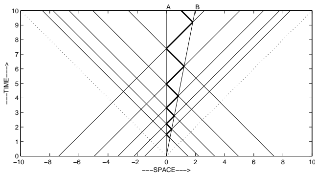
FIG. 2: Spacetime history of an inertially expanding clock and the null trajectories of trains of emitted and received pulses (light lines) whose emission and reception is controlled by the internal pulse (heavy line) bouncing back and forth between A and B.
