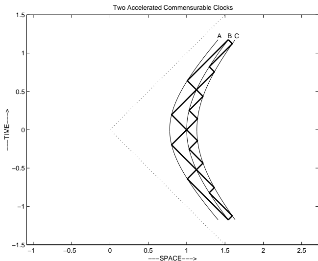
FIG. 6: Two adjacent geometrical clocks consisting of collinearly accelerated cavities AB and BC, each containing a pulse bouncing back and forth. Depicted in this diagram is a sequence of 4 pulses coming from A and impinging on B which are matched by a sequence of 8 pulses coming from C. The ratio c/a = 8/4 is the ticking rate of BC normalized to that of AB. The fact that this ratio stays constant throughout the history of the two clocks makes them also commensurable , just like those in Figure 5
