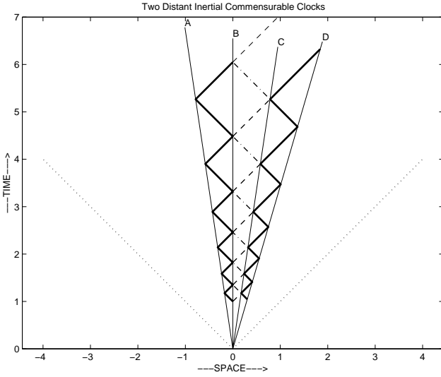
FIG. 7: Two distant inertially expanding geometrical clocks. Clock CD can be calibrated in terms of AB because CD and AB are commensurable: Taking into account the ticking rate of the intermediate clock BC, one sees that the ratio of their rates is a constant, namely 1:1. Because this ratio happens to be unity, these two commensurable clocks are said to have the additional property of being identically constructed .
