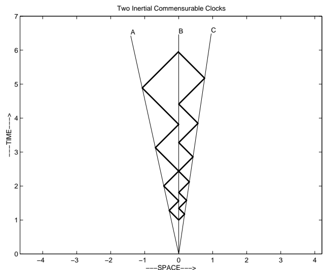
FIG. 5: Two adjacent geometrical clocks consisting of inertially expanding cavities AB and BC, each containing a pulse bouncing back and forth. Depicted in this diagram are sequences of 2 pulses coming from A and impinging on B which are matched by corresponding sequences of 3 pulses coming from C. The ratio c/a = 3/2 is the ticking rate of BC normalized to that of AB. The fact that this ratio stays constant throughout the history of the two clocks makes them commensurable .
