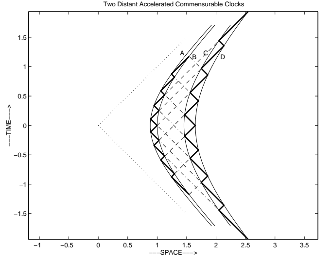
FIG. 8: Two distant accelerated geometrical clocks. Clock CD can be calibrated in terms of AB because CD and AB are commensurable: Taking into account the ticking rate of the intermediate clock BC, one sees that the ratio of their rates is \frac{1}{3} \times \frac{3}{1} = \frac{1}{1} in this figure. Because this ratio happens to be unity, these two commensurable clocks are said to have the additional property of being identically constructed .
