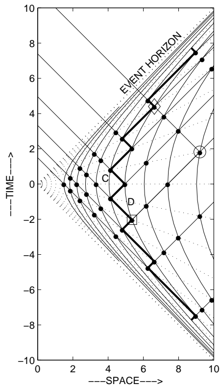
FIG. 10: Lattice of spacetime graduation events (heavy dots) as determined and calibrated by a single geometrical clock CD which is accelerating. The spacetime history of the e.m. pulse bouncing inside this clock is the heavy zig zag line between the two hyperbolas C and D. The clock is bounded by these two hyperbolas, the histories of the two accelerating reflectors which keep the e.m. pulse trapped inside the clock. The other hyperbolas indicate the accelerated reflector histories of identically constructed clocks, if they were to form an array of adjacent geometrical clocks. The straight lines (lightly dotted) are the times simultaneous with the tickings of the standard clock CD. The 45^\circ lines emanating to the left from C and to the right from D are the histories of the two trains of pulses escaping from C and D, with those escaping from C ultimately crossing the event horizon of clock CD. The fact that CD is a standard clock implies that all graduation events of the calibrated lattice lie on these histories. Based on the method of pulsed radar, each graduation event (e.g. the encircled dot) is labelled by two unique integers, namely two numbered ticks (the dots in the square and in the diamond) of the clock. They are CD's "radar coordinates" of that graduation event.
