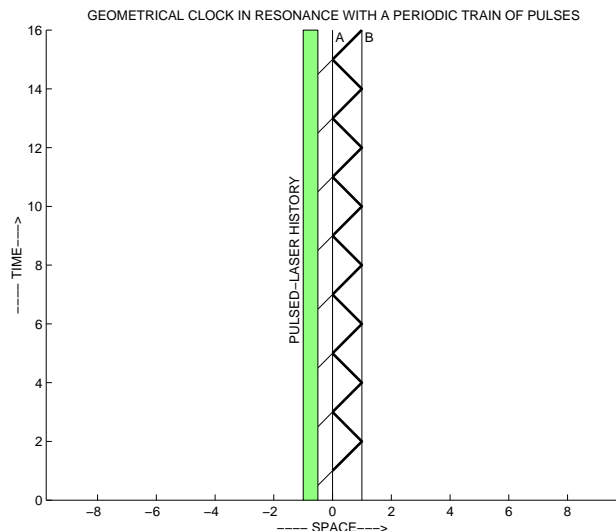
FIG. 4: Free-float geometrical clock driven at resonance by a periodic train of pulses. The partial transmissivity of partial reflector A admits part of their amplitude into the interior of geometric clock AB. When their period matches the reflection time inside the clock, resonance prevails, and they form a single pulse which bounces back and forth (heavy zig-zag line) inside AB. This bouncing is the ticking of the geometrical clock. The ticking interval is the standard of time, while the spatial extent of AB is the associated standard of length. Note that the picture omits, among others, the laser pulses reflected from A and the partially transmitted pulses emerging from B.
