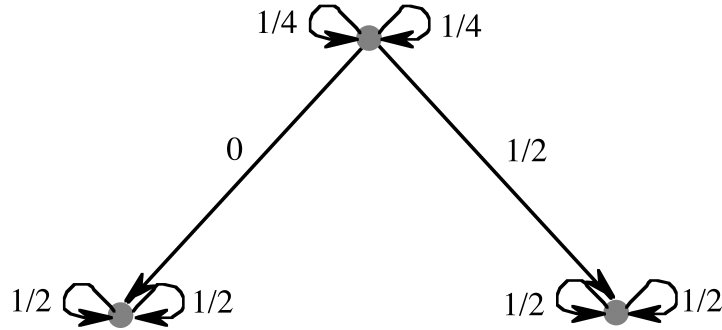
Figure 2. A Markov chain.
